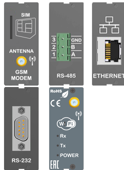
Plug-in modules
